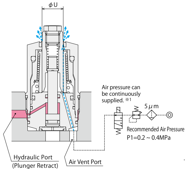
LDD Plunger Descending and at Releasing State
