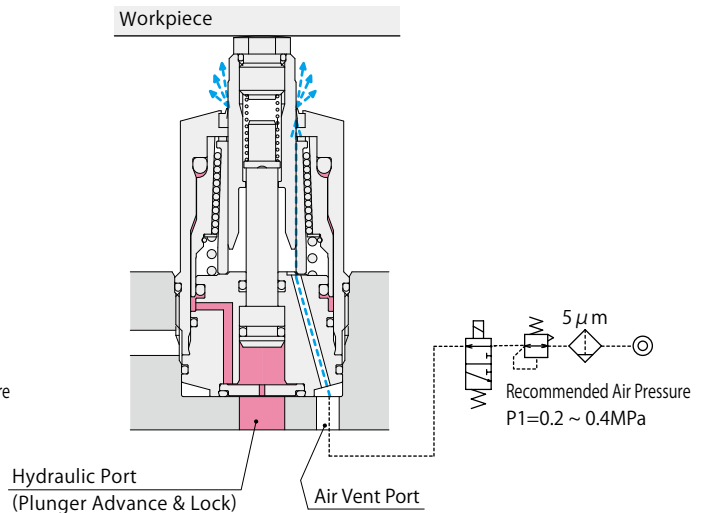
LDD Plunger Ascending and at Locking State
